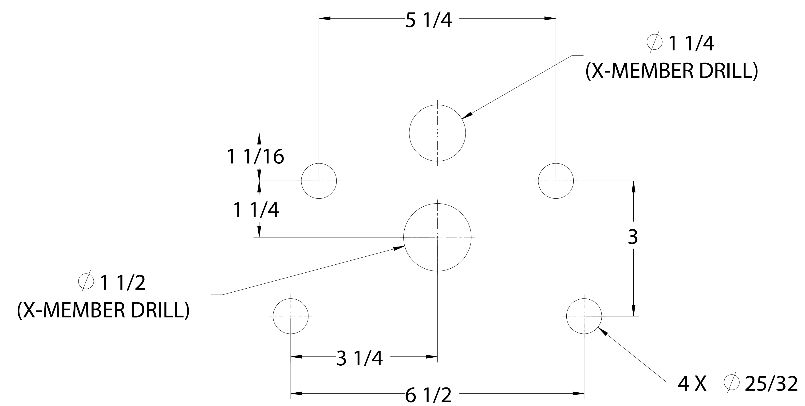
MOUNTING SURFACE DRILLING DETAIL
